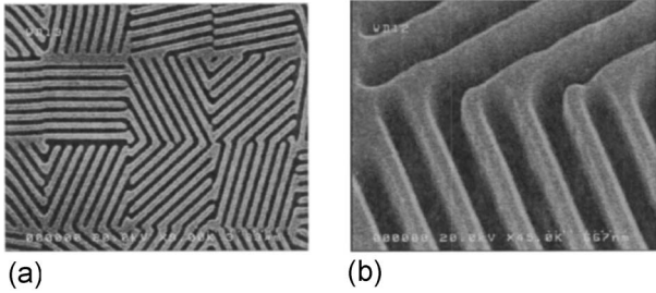
Fig. 2. SEM photograph of the fabricated F-BCGH element for operation at a wavelength of 1.55 \mu\text{m} . (a) Typical top view; (b) enlarged slanted view.
