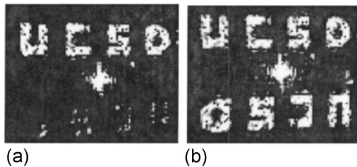
Fig. 4. Far-field reconstruction of an element operating at a wavelength of 10.6 \mu\text{m} . (a) Reconstruction achieved with right-hand circularly polarized light; (b) reconstruction achieved with linearly polarized light.
