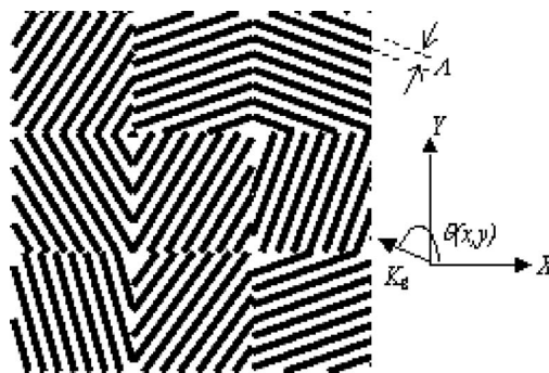
Fig. 1. Schematic diagram of the subwavelength-based array illuminator devices: A subwavelength grating with a period \Lambda is allocated into each cell. The orientation of the grating is given by \theta(x,y) .
